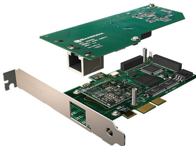
A101DE 1-port T1/E1/J1 shown with available echo canceller and PCI-Express interface
