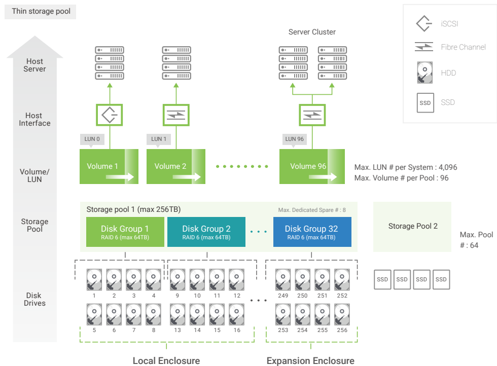
Thin Provisioning Pool Architecture
