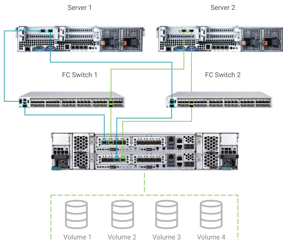
MPIO High Availability Topology for Clustered Servers
