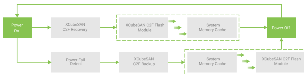
Cache-to-Flash Workflow
