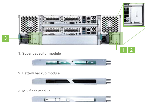
Cache-to-Flash Modules
