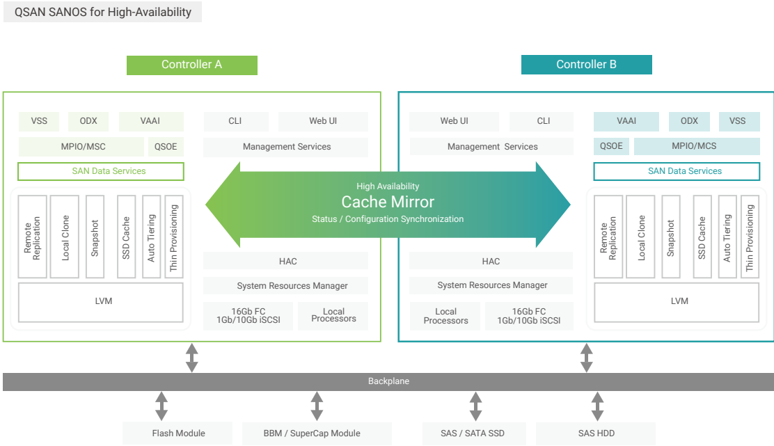
SANOS System Architecture
