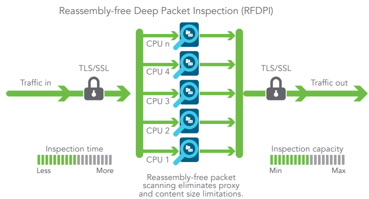
SonicWall stream-based architecture
